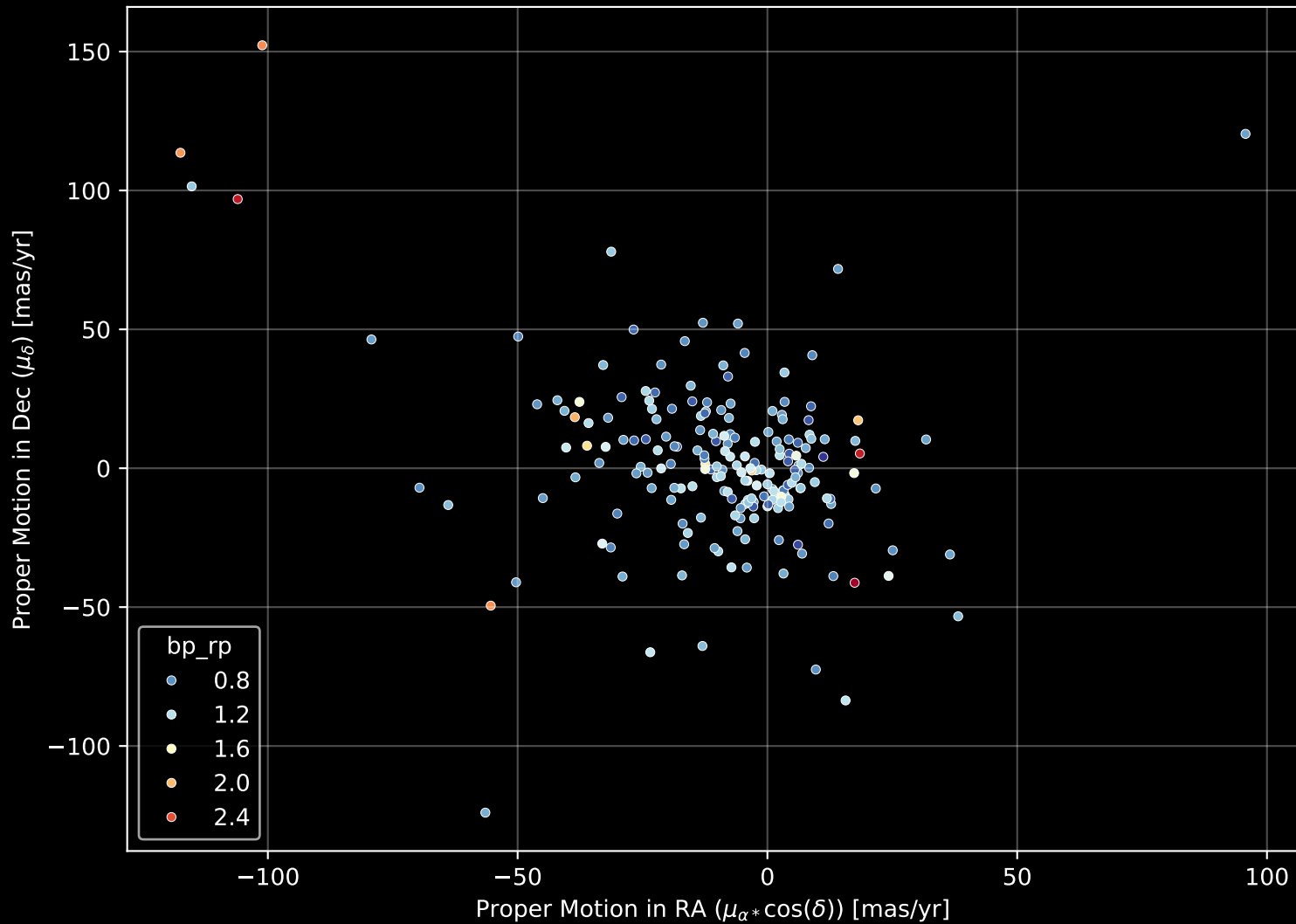
APOGEE DR17 Field: [079+47_MGA] Proper Motion Diagram (n= 204)
