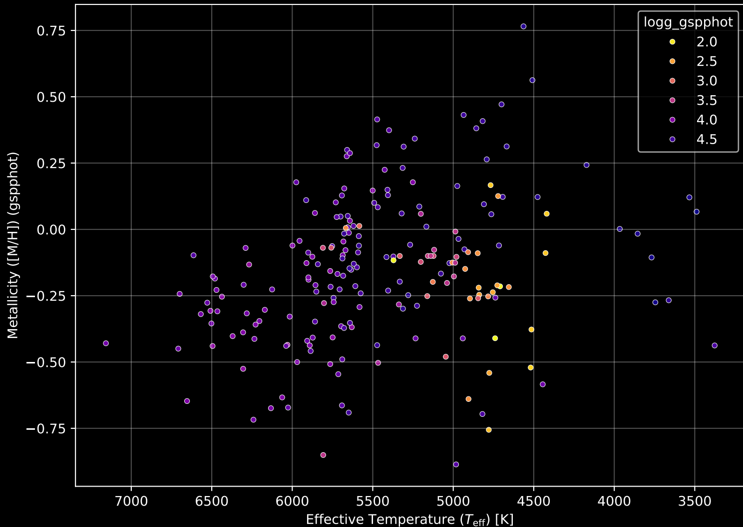
APOGEE DR17 Field: [079+47_MGA] Stellar Population Parameters (n= 204)
