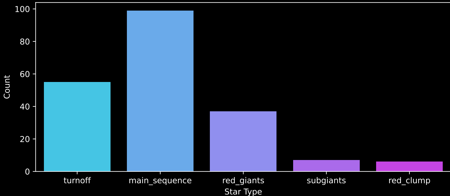
APOGEE DR17 Field: [079+47_MGA] Count plot of Star Type
