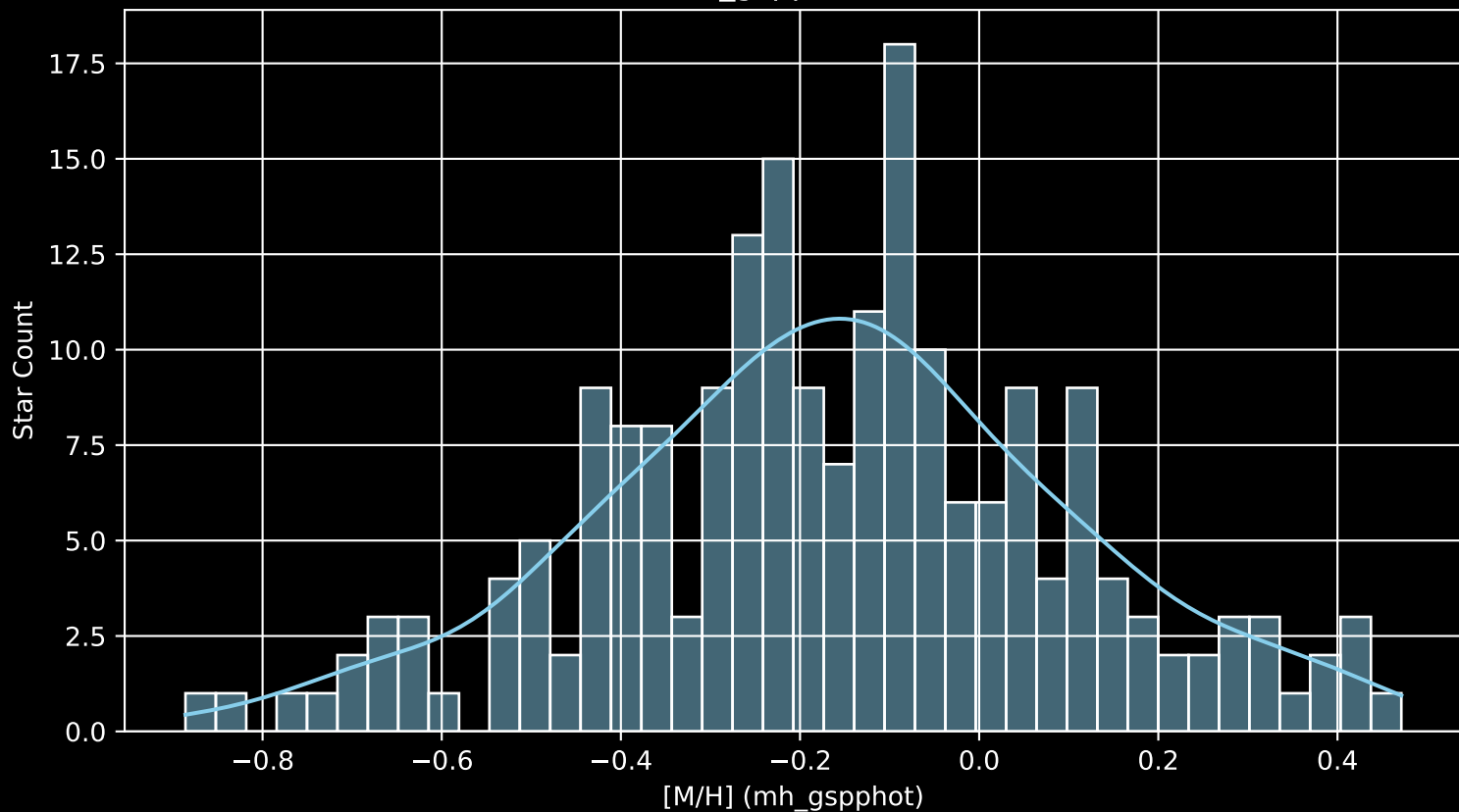
APOGEE DR17 Field: [079+47_MGA [M/H] (mh_gspphot) (n= 202)
