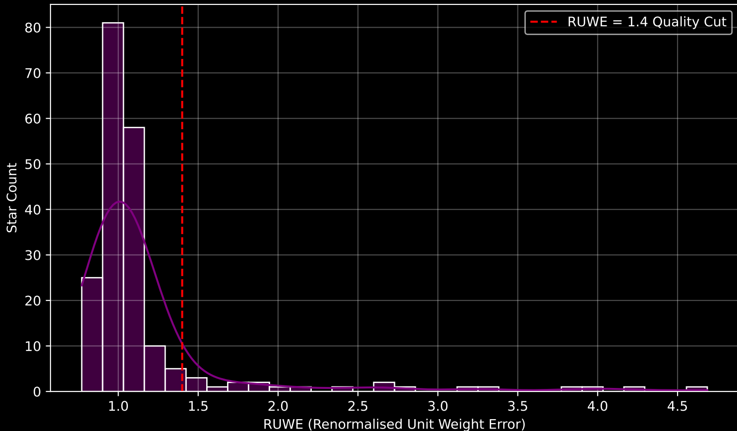
GAPOGEE DR17 Field [079+47_MGA] RUWE Distribution (n= 199)
