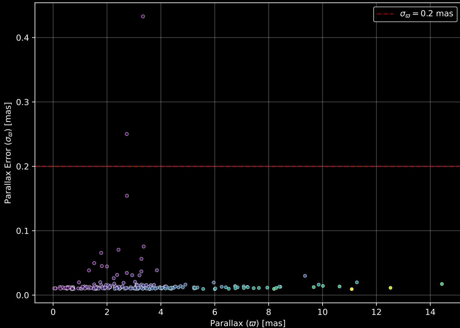
APOGEE DR17 Field: [079+47_MGA] Parallax Quality (n= 204)
